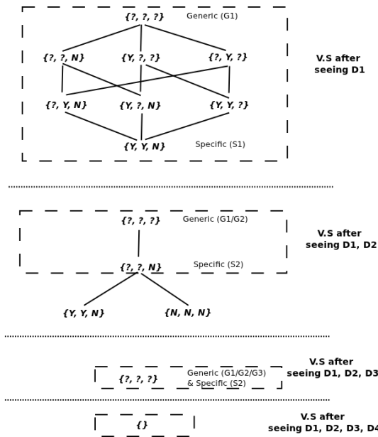
Figure 3: Progressive construction of Version Spaces for table 1
